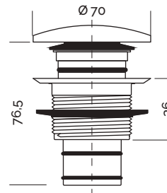
Bonde click-clack Dolotek (mm)
